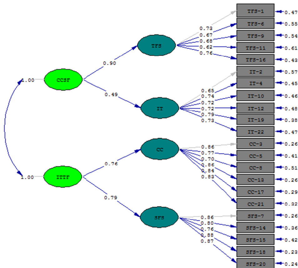
Figure 1. Parameters of standardized CFA
