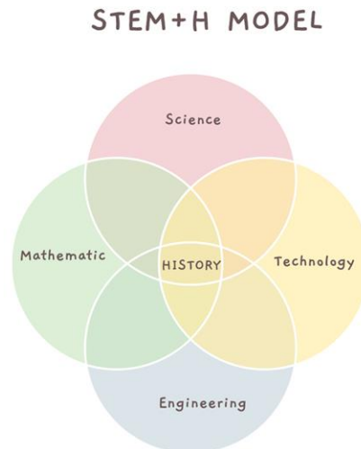
Figure 1. STEM+H model
