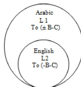
Figure 3. L1 is the superset and L2 is the subset
