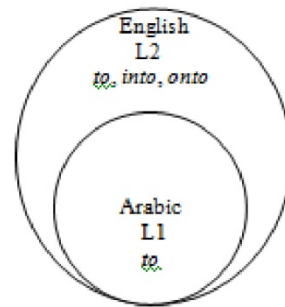
Figure 4. L2 is the superset and L1 is the subset
