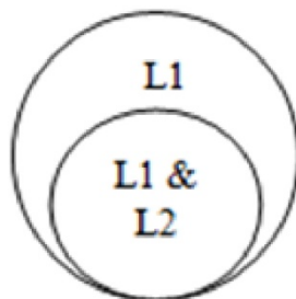
Figure 1. L1 superset - L2 subset relationship
