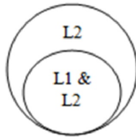
Figure 2. L2 Superset - L1 subset relationship
