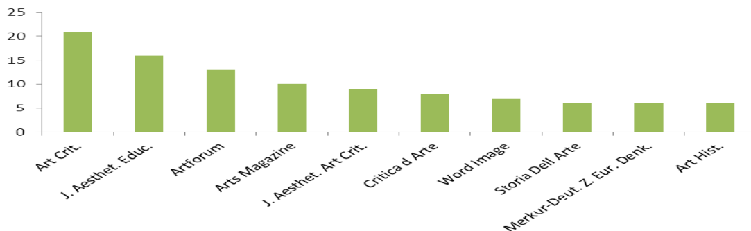
Figure 3. The top 10 journals that published the topmost number of the 214 articles
