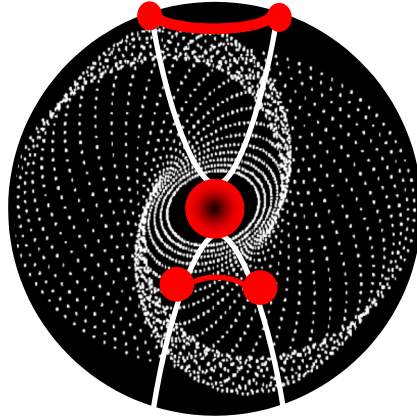
Figure 10. All these variables help to create shapes in galaxies like the golden spiral ( \varphi = 1,6180 )
