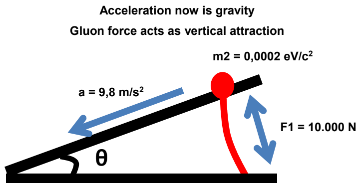
Figure 5. Inclined plane forces (gluon catching strings)
