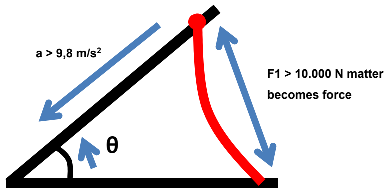
Figure 7. Increase the separation, increase the force exerted. Matter is transformed into energy
