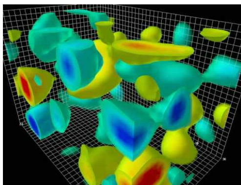
Figure 3. Gluon into vacuum (Special Research Centre for the Subatomic Structure of Matter)
