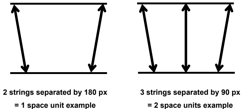
Figure 1. String example
