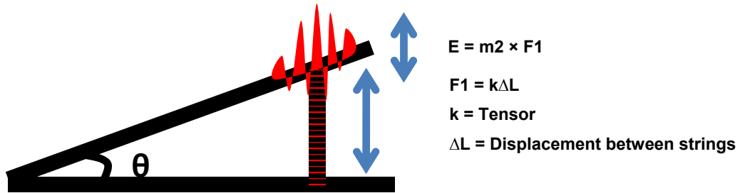
Figure 8. Energy don't disappear becomes matter
